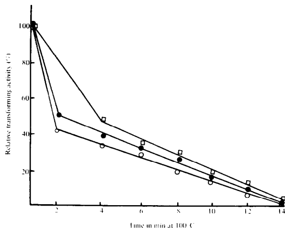
Fig. 2. Heat inactivation of the arginine, histidine and tryptophan genes at 100^\circ\text{C} . DNA was thermally denatured at a concentration of 20\ \mu\text{g/ml} in 0.15\ \text{M} NaCl containing 0.02\ \text{M} potassium phosphate buffer, pH 6.8, for different intervals of time and immediately cooled in an ice-bath. Transforming activity was carried out at a DNA concentration of 1\ \mu\text{g/ml} using competent strain of B. subtilis (histidine ^- , tryptophan ^- , arginine ^- ) prepared as described previously [5]. The activity values are shown as percentage of the original native DNA. ●—● histidine gene; ○—○ tryptophan gene; □—□ arginine gene.
